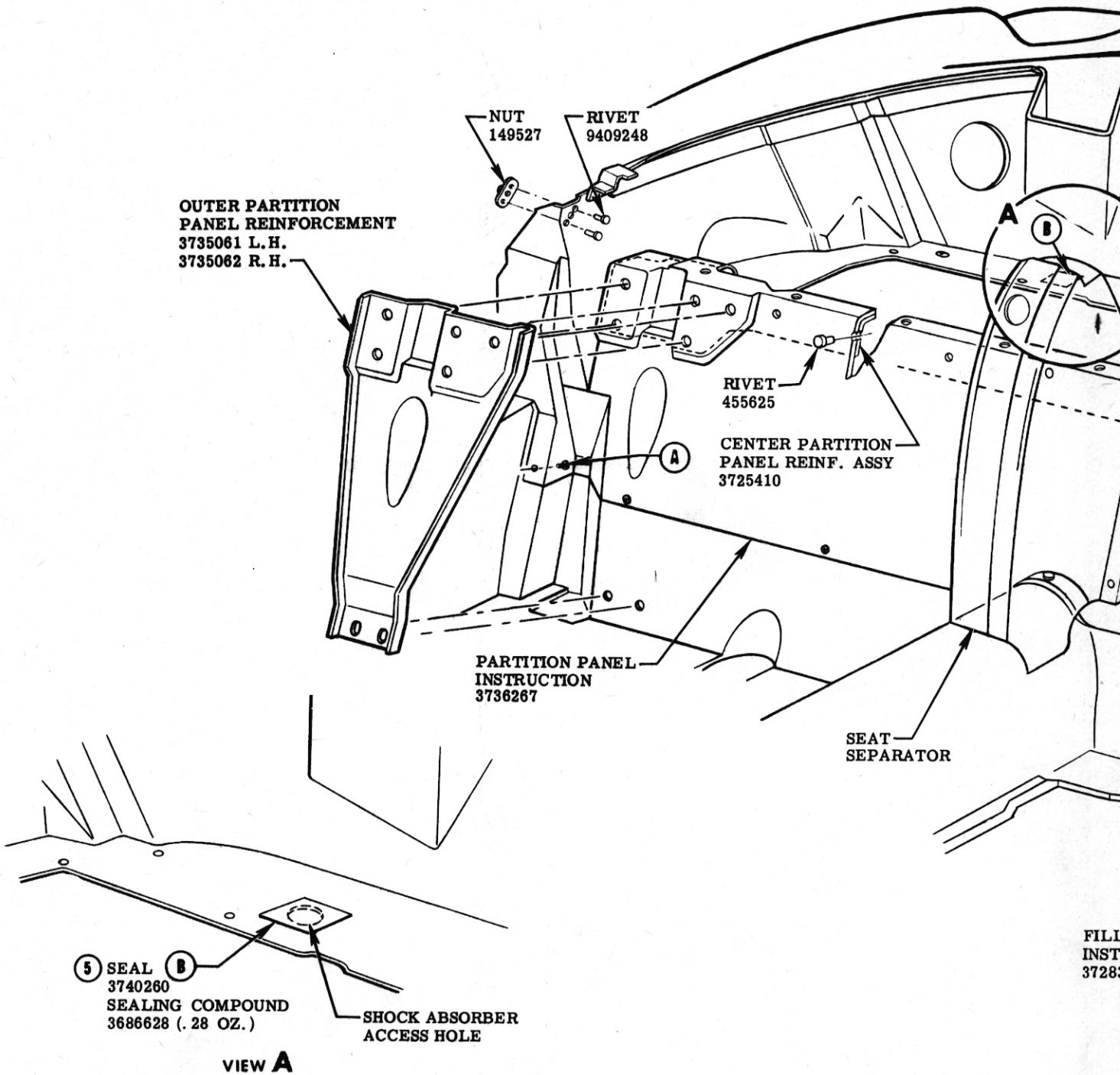
SEAT BACK PARTITION PANEL & FILLER PANEL
