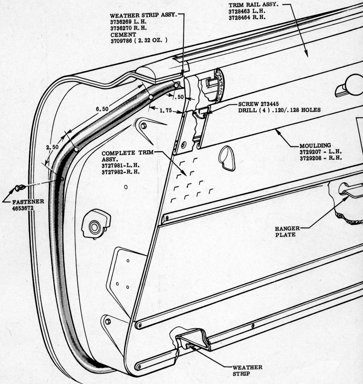
TRIM PANEL, MOULDING & WEATHER STRIPS
