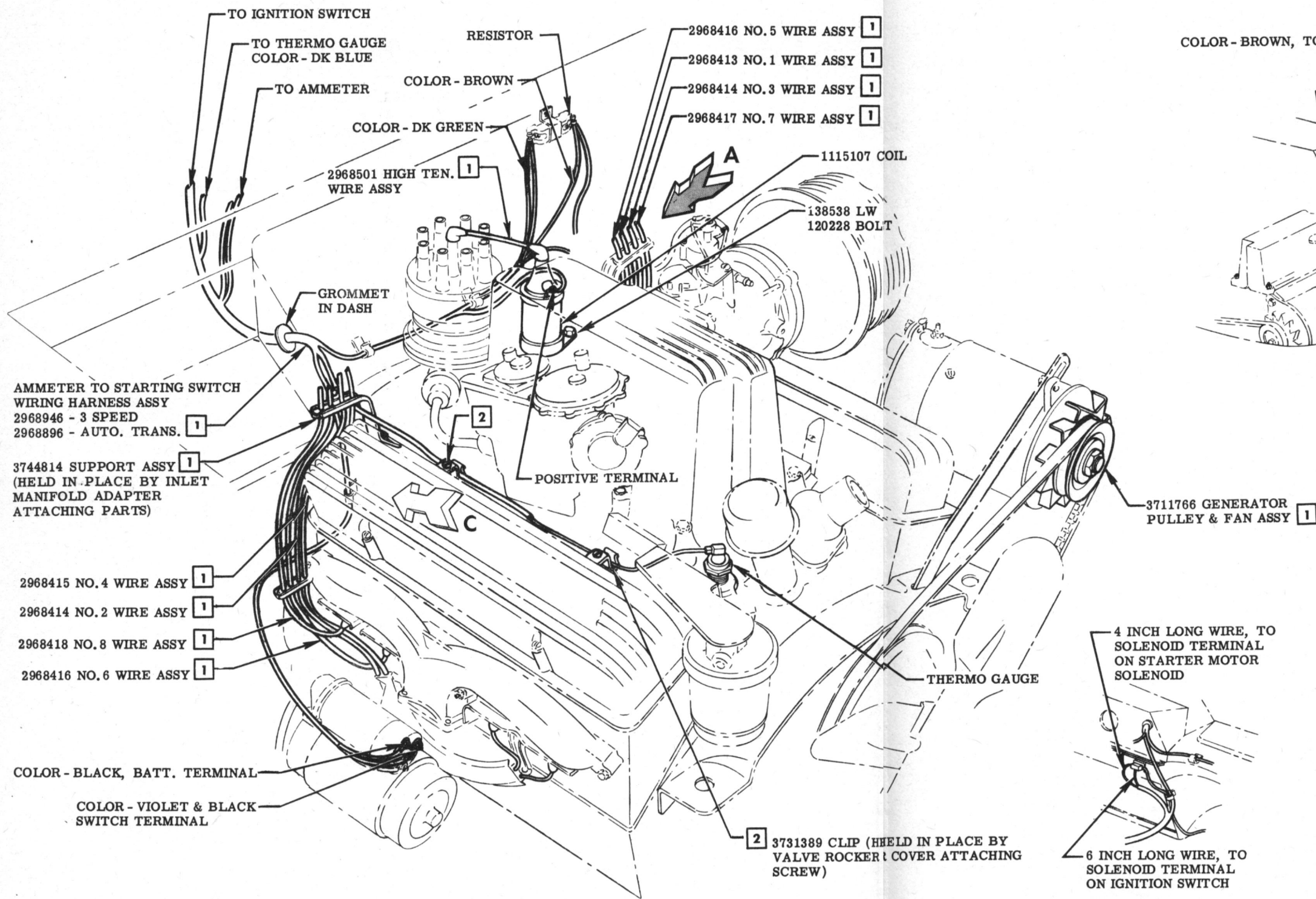
VIEW C RPO 313 ONLY
