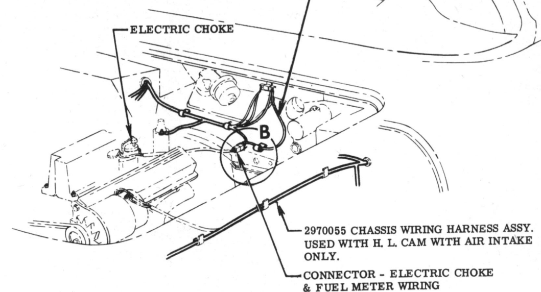
VIEW A
