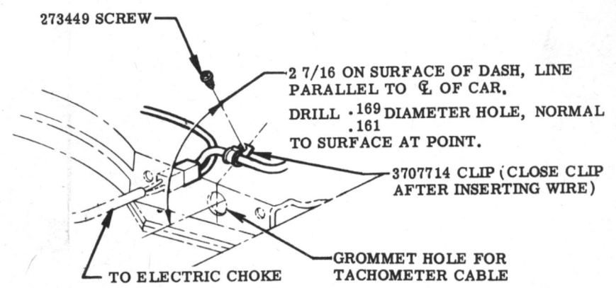
VIEW B
